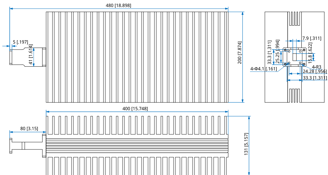
Outline A
